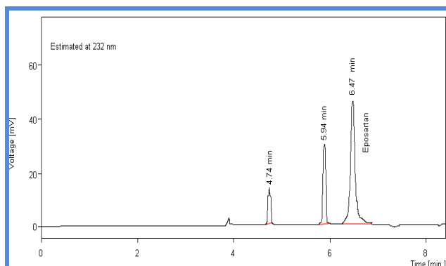
Figure 7: The simple chromatogram of UV degraded sample.
