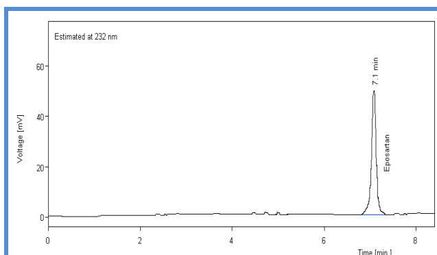
Figure 2: The simple chromatogram of standard Eprosartan.
