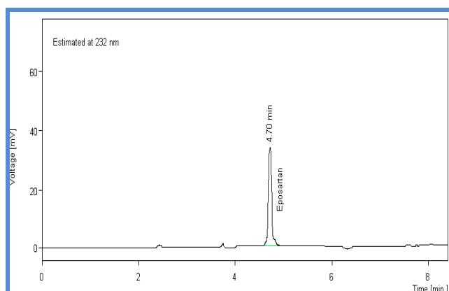
Figure 7: The simple chromatogram of Thermal degraded sample.
