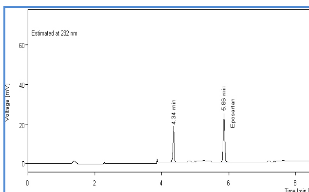
Figure 5: The simple chromatogram of alkali degraded sample.
