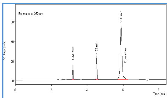
Figure 6: The simple chromatogram of Hydrogen Peroxide degraded sample.
