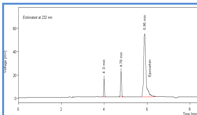
Figure 4: The simple chromatogram of acid degraded sample.
